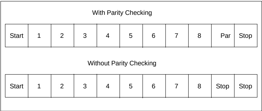
Figure 6 Bit Order (RTU)
